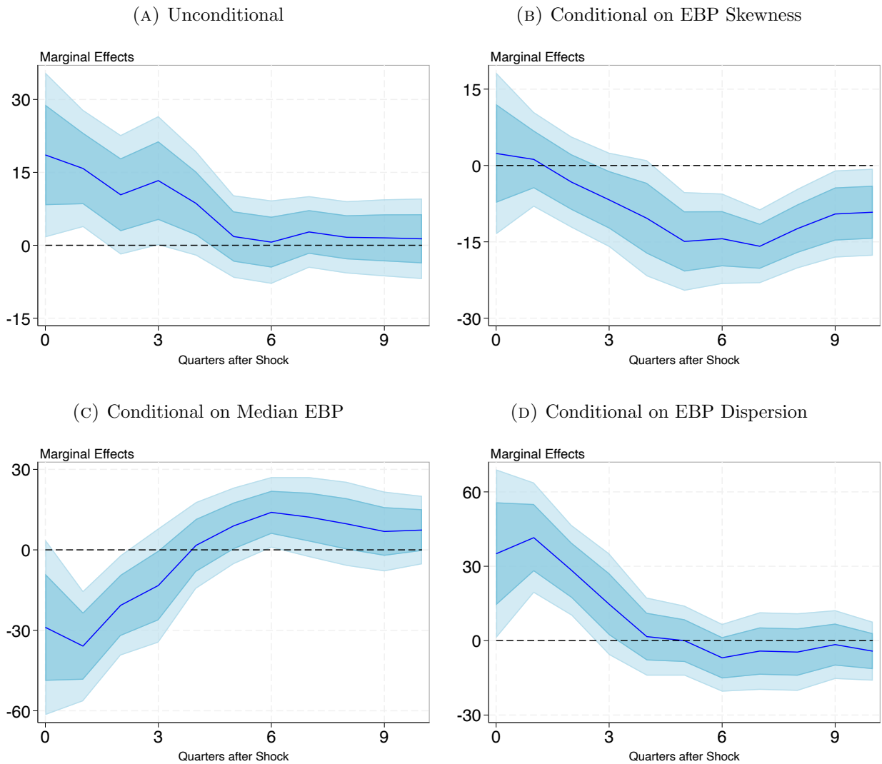
FIGURE B.19 Monetary Policy's Effect on Aggregate Investment Growth Horseshoe between EBP moments and NBER Recession Indicator
