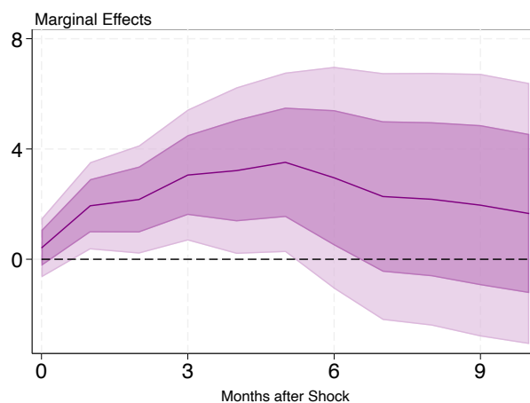
(E) Below 50 th EBP_{ikt-1} Percentile
