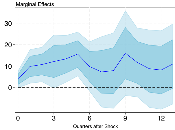
(E) Below 50 th EBP_{it-1} Percentile
