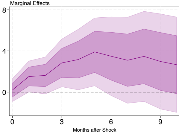
(C) Below 33 rd EBP_{ikt-1} Percentile
