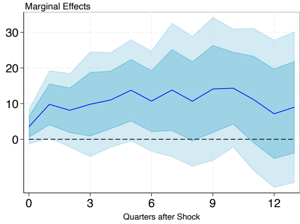
(B) Below 15 th EBP_{it-1} Percentile
